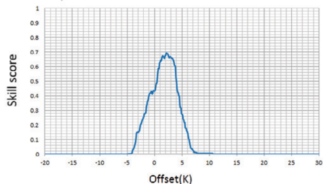
Fig. A-1. Bias values for T39T112opaque and skill scores. This test is for opaque cloud detection at nighttime using T(3.9) - T(11.2) as described in 3.1.2.
