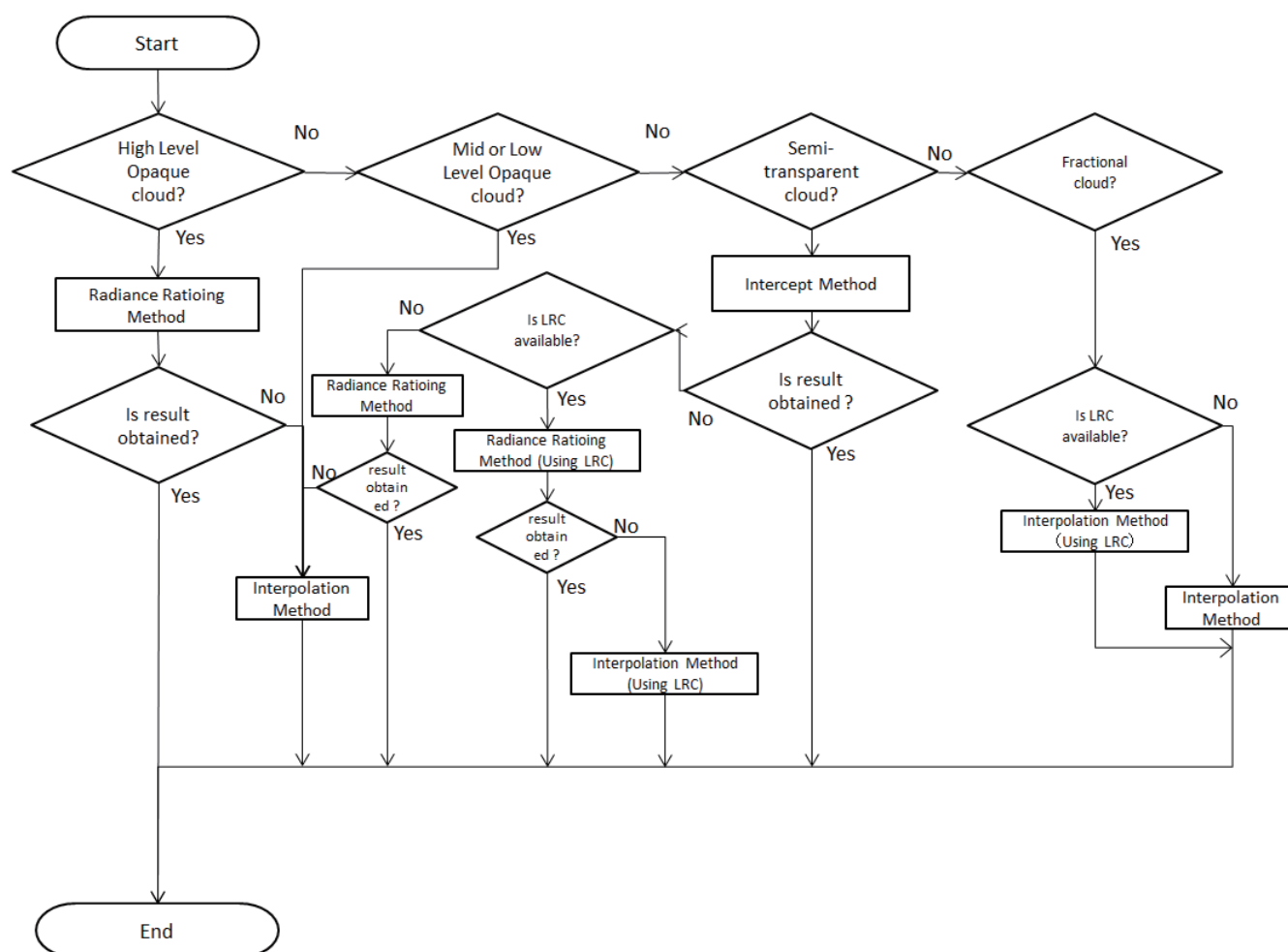
Fig. 1 Process flow of the cloud top height product
